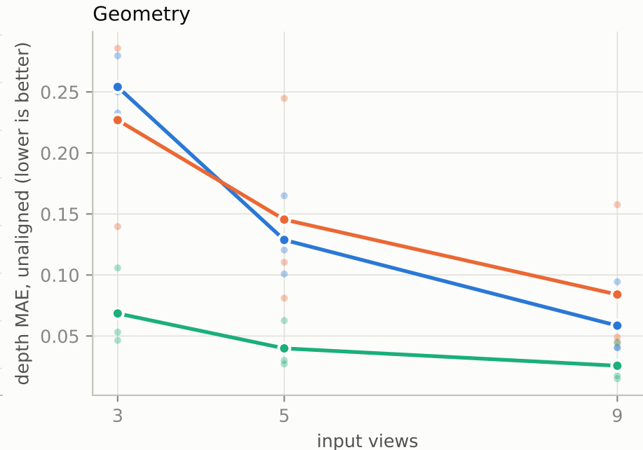
Initialization vs view count, no depth loss — mean over scenes, faint dots are single scenes (fps split, SH 0, 7000 iters)
