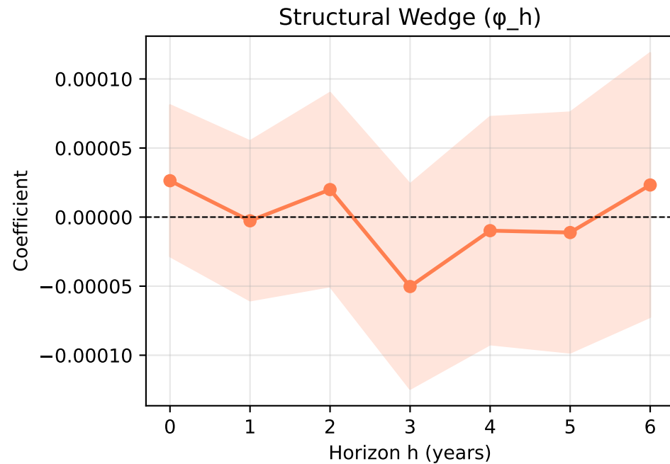
Panel LP Interaction Coefficients (shock \times moderator)
