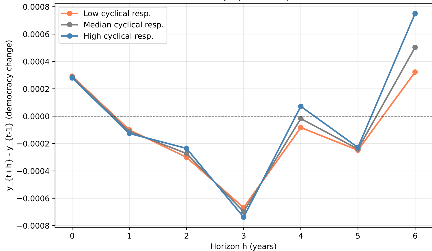
IRFs to -1\sigma GDP Shock by Cyclical Responsiveness Tercile
