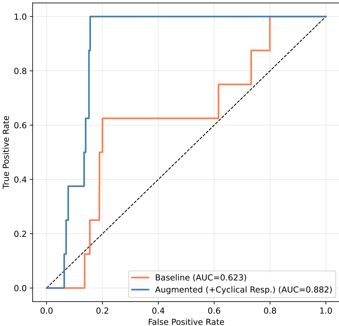
ROC Curves: Backsliding Prediction
