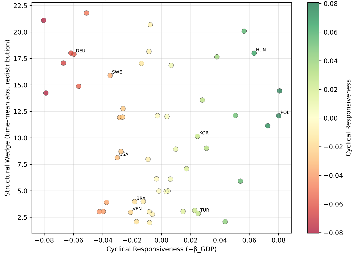
Country Decomposition: Cyclical vs. Structural Redistribution
