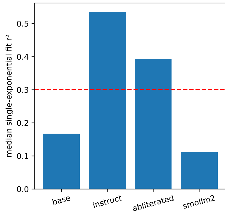
A. Fit quality ( r^2 = 0.3 marked)
