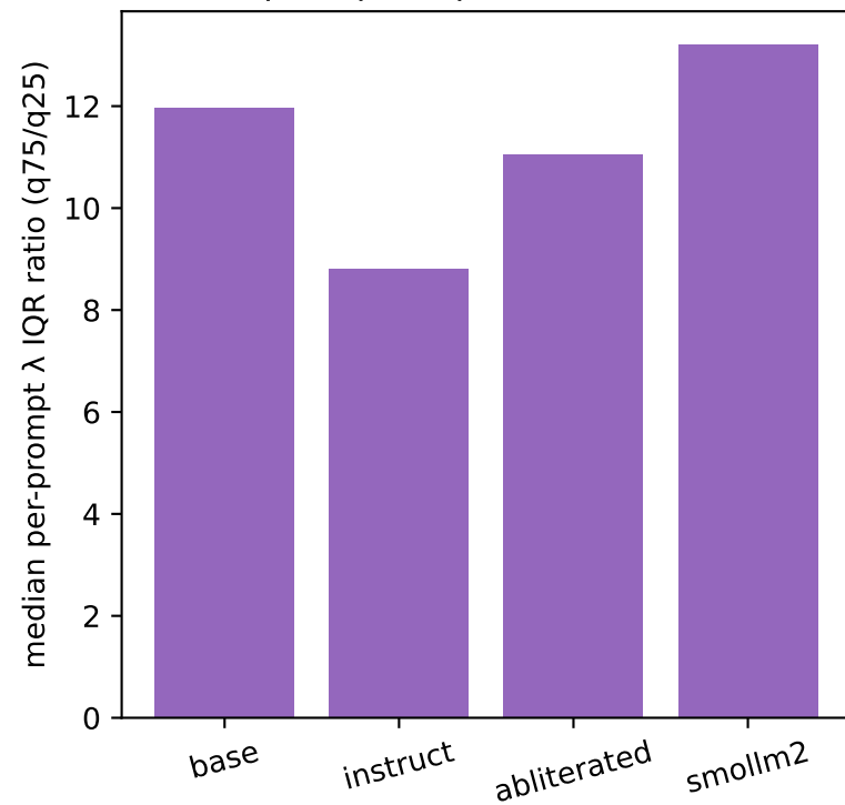
C. Within-prompt \lambda spread across 20 rollouts
