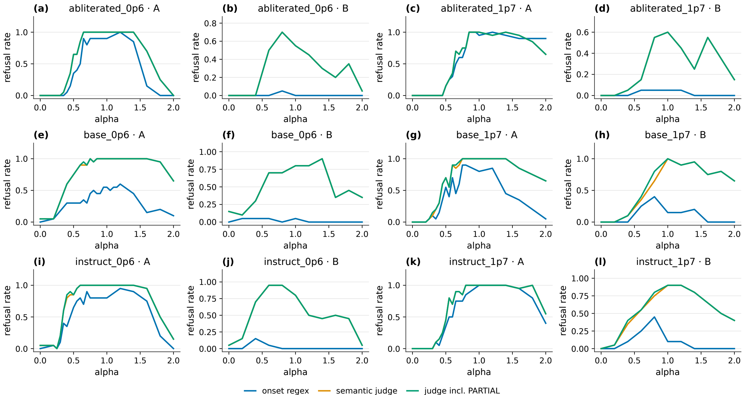
Dose response under the onset regex vs the semantic judge (alpha in NORM_L units)
