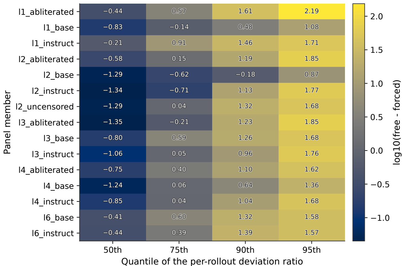
Free-running minus teacher-forced deviation ratio, by quantile (all 60 cells positive; log scale)
