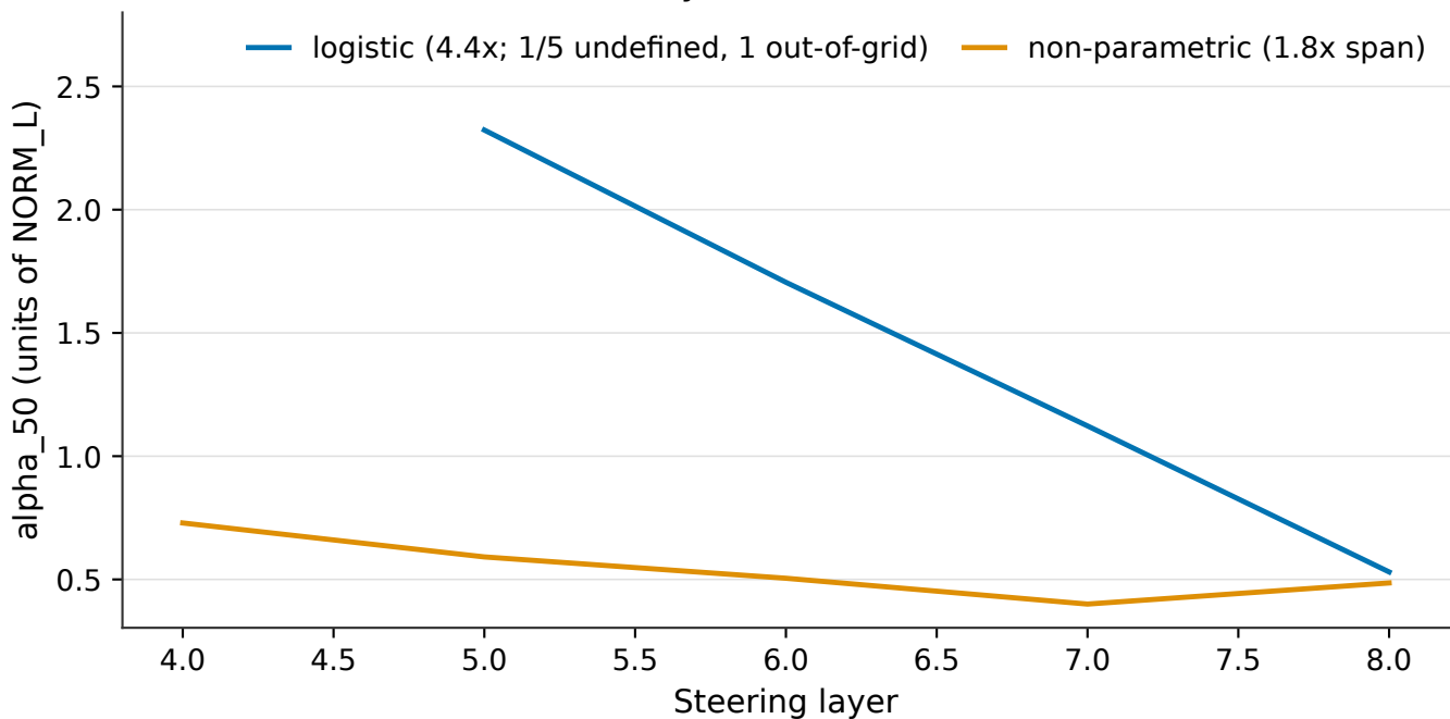
Layer sensitivity of alpha_50, l1_instruct (L=6); dose curve non-monotone at layers 4, 5, 6, 7
