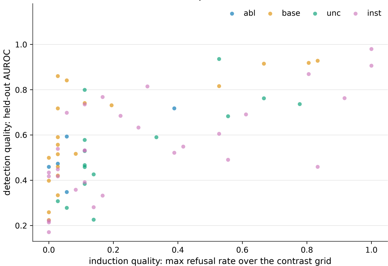
Reading versus pushing: \rho = 0.63 [0.46, 0.80] over 70 (member, axis) pairs
