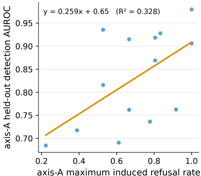
(a) Within axis A, across 14 models: \rho = 0.547
