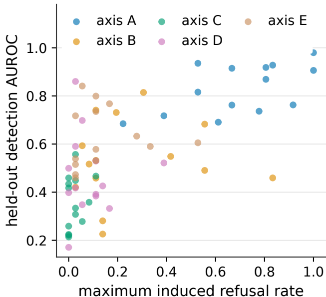
(b) Pooled over all 5 axes (70 pairs): \rho = 0.629
