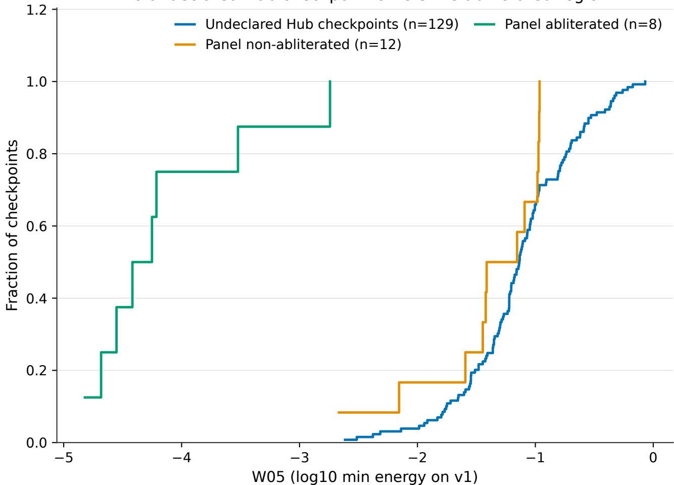
No undeclared Hub checkpoint enters the abilitated region
