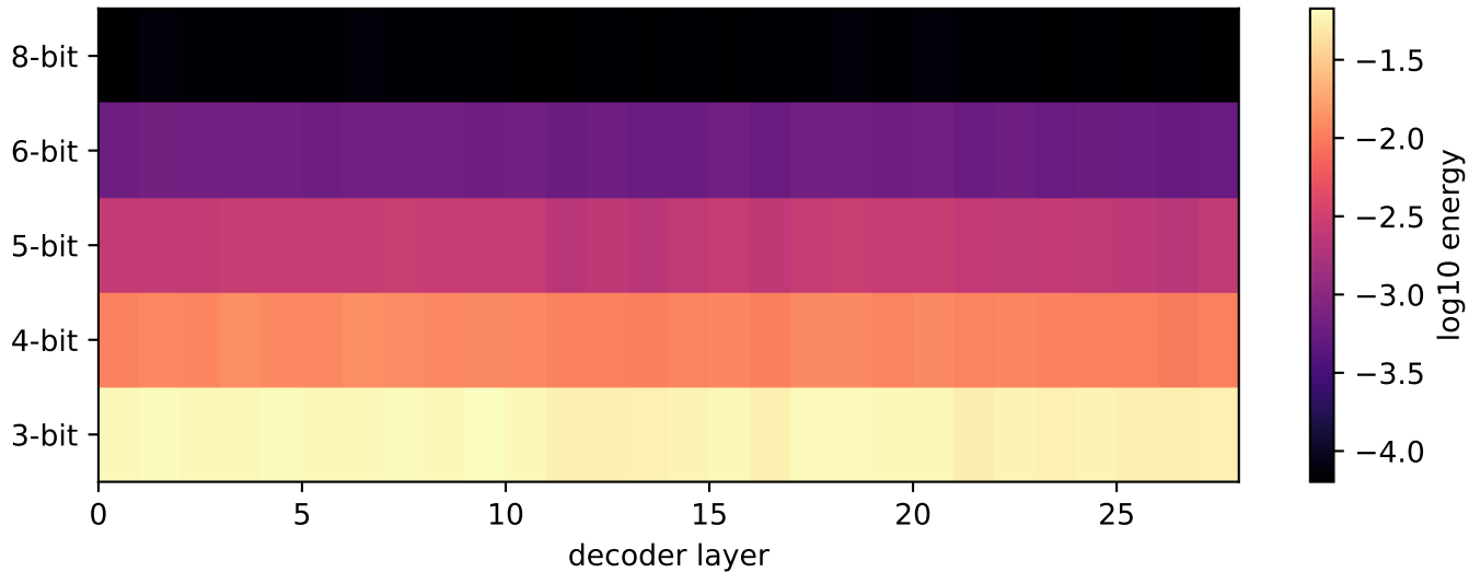
per-layer log10 min v1 energy: which layers lost the suppression
