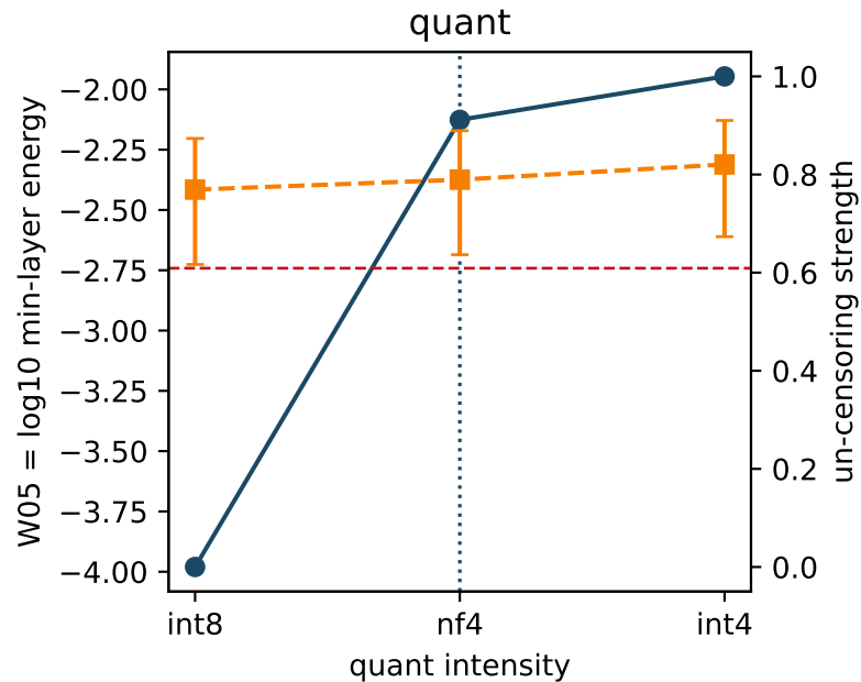
root A (Qwen/Qwen3-1.7B): flag death vs un-censoring death
