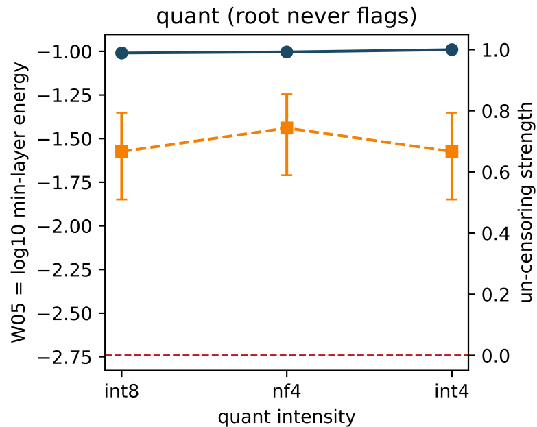
root B (Qwen/Qwen3-1.7B): flag death vs un-censoring death
