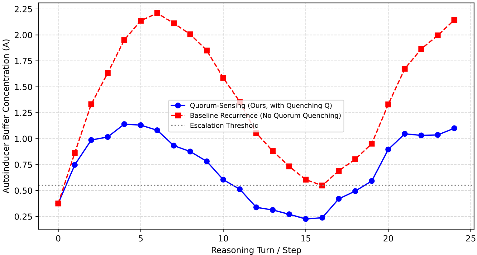
Autoinduction Buffer Dynamics & Quorum Quenching Damping
