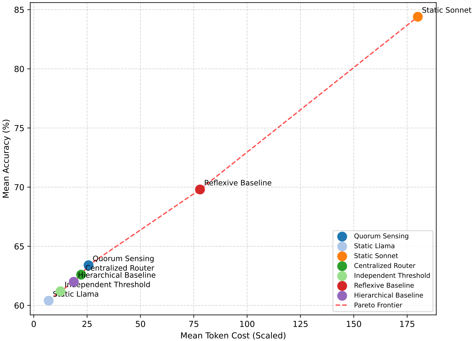
Pareto Efficiency: Accuracy vs Token Cost
