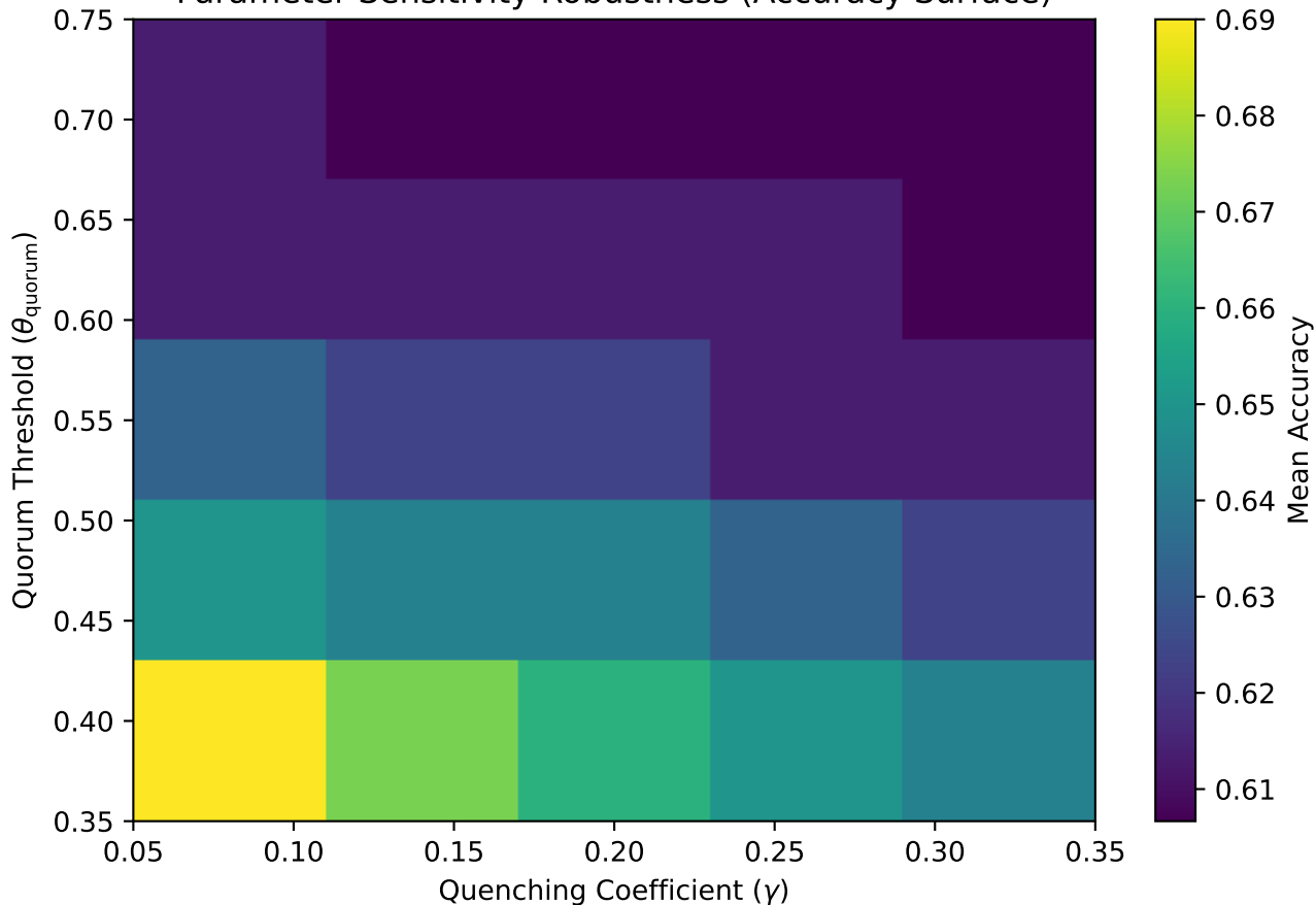
Parameter Sensitivity Robustness (Accuracy Surface)
