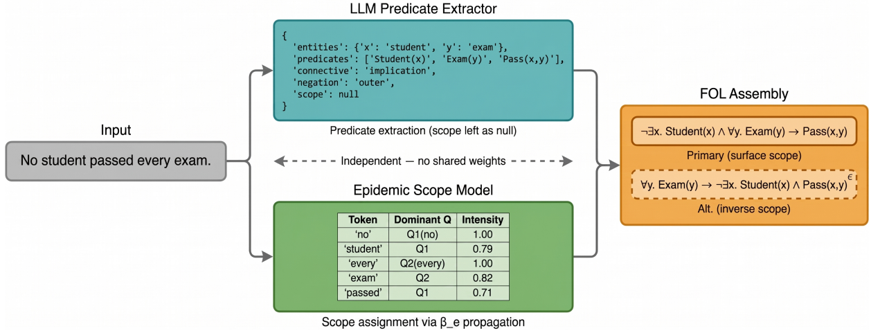
Figure 1: Detailed view of the neuro-symbolic interface. The LLM returns a structured JSON with predicate names, arities, and entity variables but with scope left as null . The epidemic scope model fills in the quantifier nesting and variable binding to produce the final FOL formula. For contested sentences, two formulas are assembled simultaneously.
