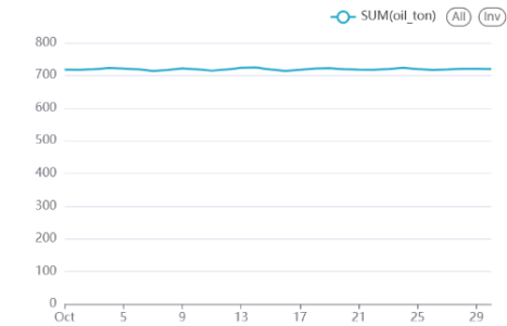
mining_by_time
