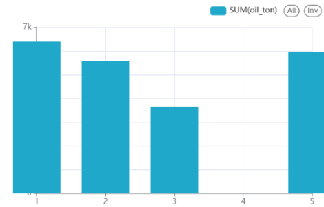
top wells
