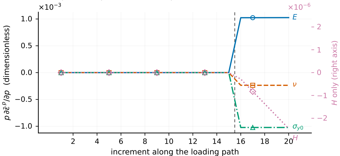
(b) Equivalent plastic strain response to each material constant
