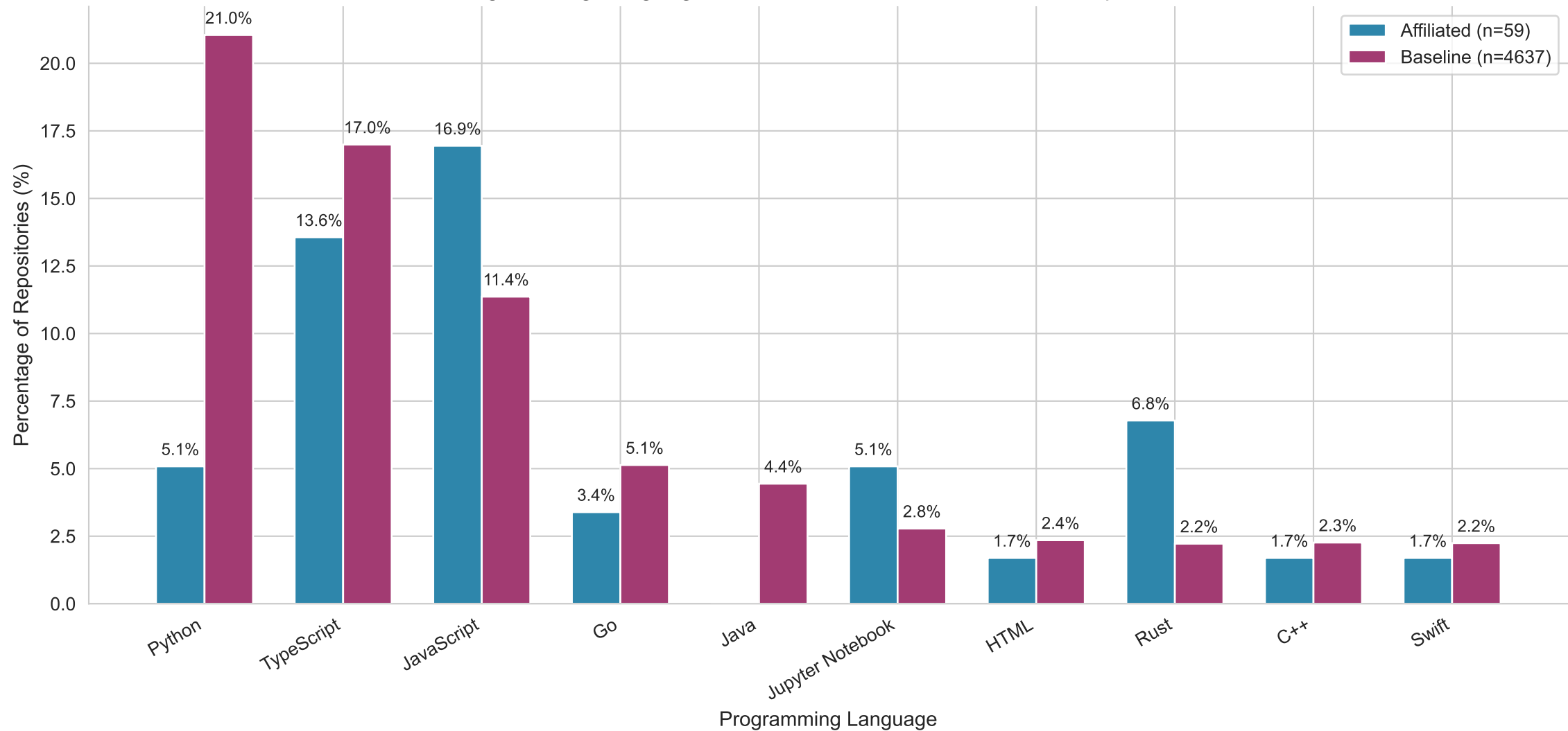
Programming Language Distribution: Affiliated vs Baseline Repositories
