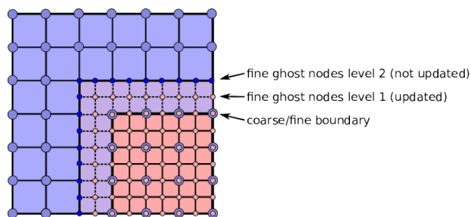
Fig. 10.1: Reflux-free coarse-fine boundary update. Level 2 ghost nodes (small dark blue) are interpolated from coarse boundary. Level 1 ghost nodes are updated during the relaxation along with all the other interior fine nodes. Coarse nodes (large blue) on the coarse/fine boundary are updated by restricting with interior nodes and the first level of ghost nodes. Coarse nodes underneath level 2 ghost nodes are not updated. The remaining coarse nodes are updated by restriction.
