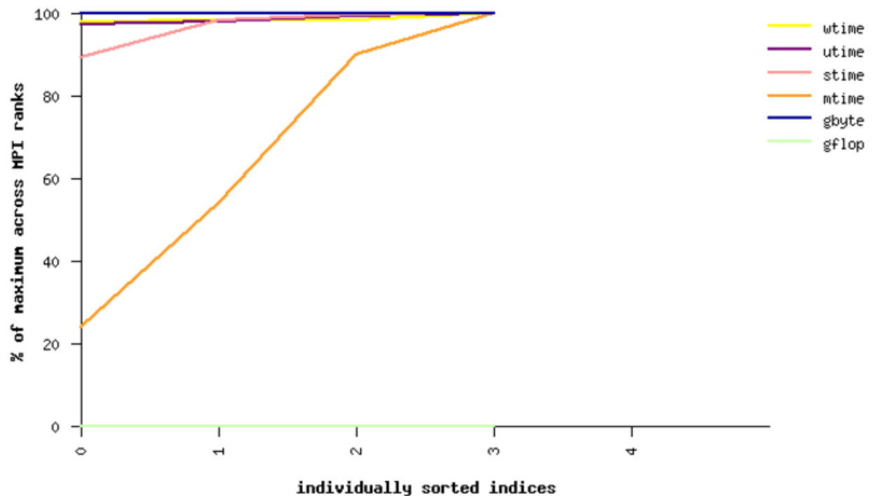
Fig. 23.1: Sample performance summary generated by IPM
