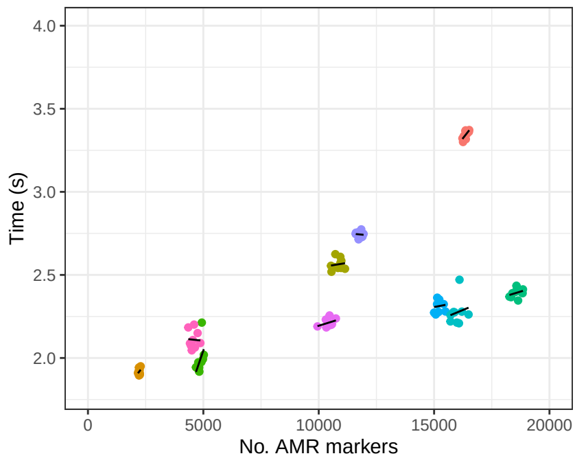
b) Runtime vs no. AMR markers for subsets of n=1000 samples
