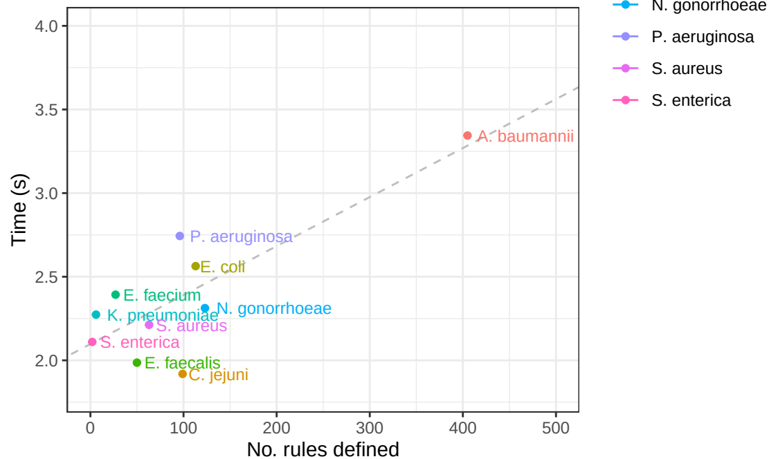
c) Runtime vs no. rules defined for subsets of n=1000 samples
