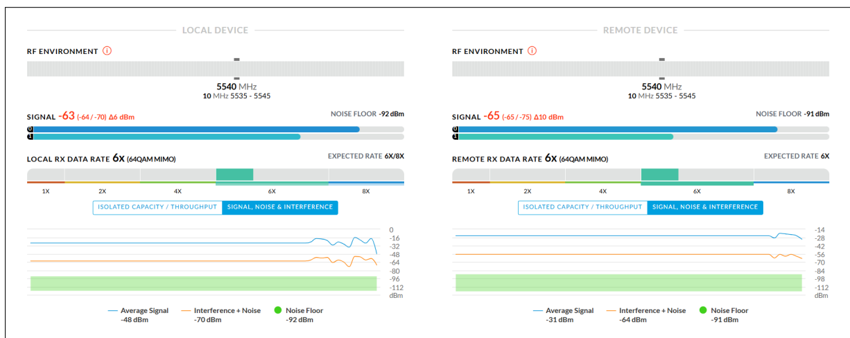
Figura 27: Panel principal desalineado (10 MHz)
