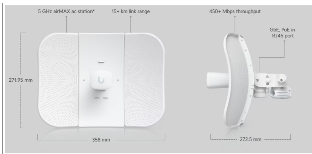
Figura 6: Vista frontal y lateral Ubiquiti LiteBeam 5AC Gen2 .
