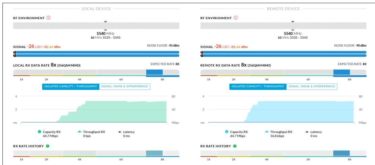
Figura 25: Panel principal alineado (10 MHz)
