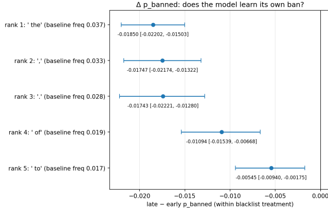
Figure 1: With one token banned during generation, the model’s predicted probability on the banned token falls across the sequence (late minus early, \Delta p = -0.019 for the top token) and below an unbanned control, evidence the model has inferred the blacklist from its own text.
