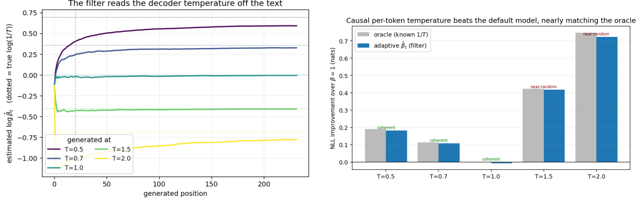
Figure 2: Beat 2. Left : on known-temperature self-text the streaming \hat{\beta}_t recovers the true \log(1/T) from the prefix alone. Right : using \hat{\beta}_t as a per-token temperature lowers held-out NLL toward the oracle that knows 1/T . (Large T \geq 1.5 gains are on near-random text; coherent wins are at T=0.5, 0.7 .)
