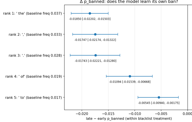
Figure 1: Beat 1. With one token banned during generation, the model’s predicted probability on the banned token falls across the sequence (late minus early, \Delta p = -0.019 for the top token) and below an unbanned control — evidence the model has inferred the blacklist from its own text.
