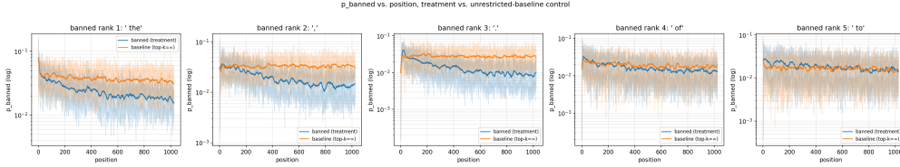
Figure 1: Model probability assigned to the banned token vs. sequence position, per banned rank. Probability mass on a commonly-banned token decays as the model infers the ban from its absence in the context.
