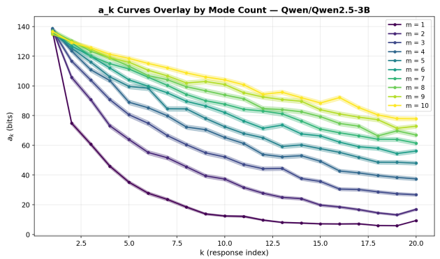
Figure 5. Mode count scaling on Qwen2.5-3B ( n = 20 , 1000 draws). The a_k curves fan out with increasing m : higher floors, slower convergence. All curves are exponential (no sigmoidal plateau), even at m = 10 , due to cross-mode learning (Section B.4).
