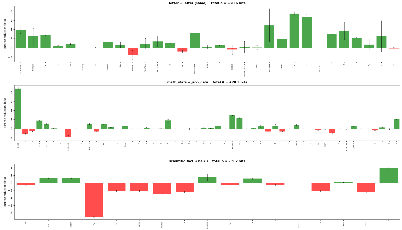
Figure 9. Per-token surprise reduction (bits) for three representative context–target pairs (Qwen2.5-3B). Bars are mean reductions across 5 context samples per pair; error bars are \pm 1 standard deviation. Green bars indicate the conditioning context lowered the per-token surprise; red bars indicate it raised it. The three pairs are stratified-median selections (by total |\Delta| ) from the same-mode, positive cross-mode, and negative cross-mode strata of a 9-pair pool. Note how in scientific fact to haiku, the early newline triggers the largest surprise. Scientific facts may discuss “still water”, but they almost never have a line with three words in it.
