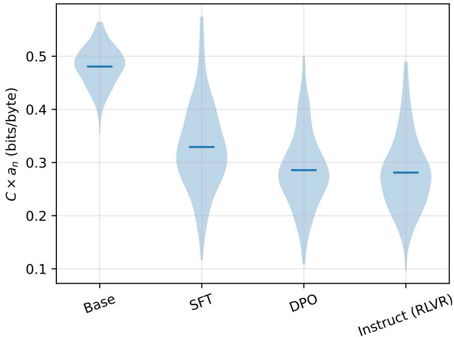
Per-prompt diversity on alpacaeval
