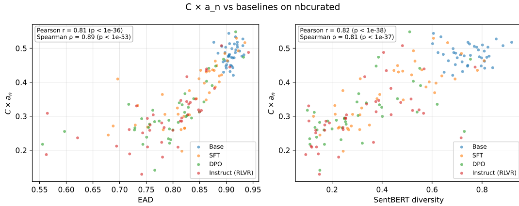
Figure 18. Per-prompt D_{Ca_n} versus EAD (left subpanel) and SentBERT-similarity diversity (right subpanel), coloured by stage, on the length-matched subset of prompts. Length-matching truncates each (stage, prompt) tuple’s responses to a common per-prompt byte budget so the per-byte conditional surprise that defines a_n is not depressed by response length. Pearson r and Spearman \rho (two-sided p ) are reported in each panel. The rank correlations are positive across both prompt sets and both baselines: D_{Ca_n} tracks the same diversity-loss signal EAD and SentBERT detect, and the agreement is not an artefact of response length.
