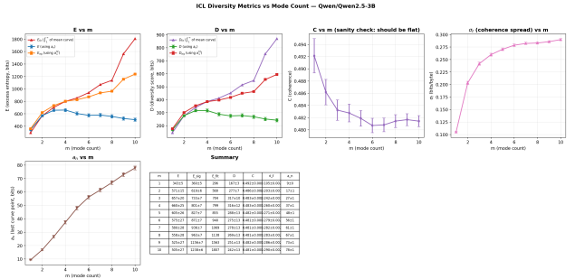
Figure 13. Summary metrics vs. mode count m (Qwen2.5-3B, n = 20 , 1000 draws). E_{fit} (sigmoid-extrapolated) increases monotonically, while the raw \hat{E}_n does not.
