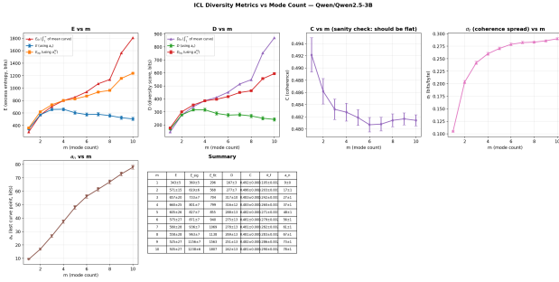
Figure 13. Summary metrics vs. mode count m (Qwen2.5-3B, n = 20, 1000 draws). E_{\text{fit}} (sigmoid-extrapolated) increases monotonically, while the raw \bar{E}_n does not.
