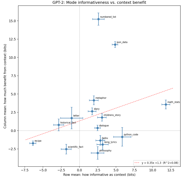
(b) GPT-2: slope = 0.35, R^2 = 0.08 .
