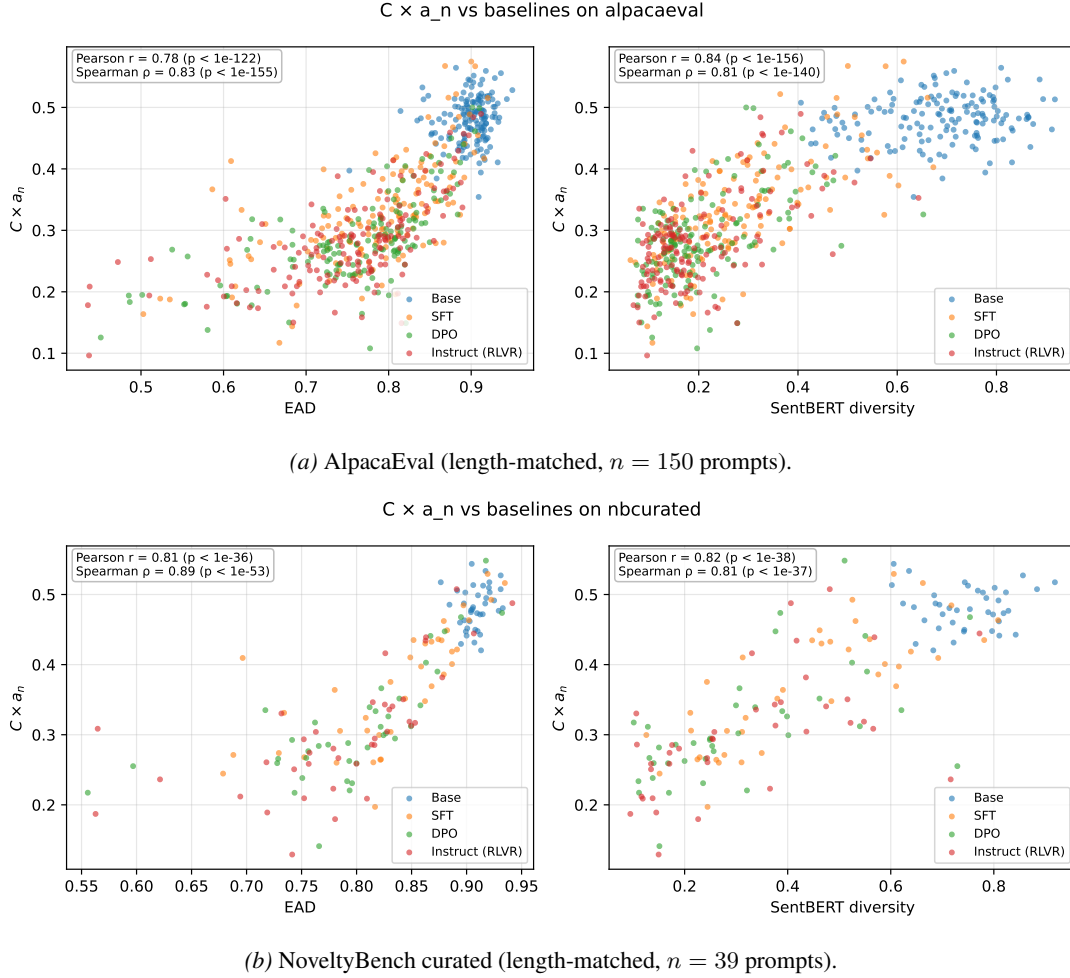
Figure 3. Per-prompt D_{C a_n} versus EAD (left subpanel) and SentBERT-similarity diversity (right subpanel), coloured by stage, on the length-matched subset of prompts. Length-matching truncates each (stage, prompt) tuple’s responses to a common per-prompt byte budget so the per-byte conditional surprise that defines a_n is not depressed by response length. Pearson r and Spearman \rho (two-sided p ) are reported in each panel. The rank correlations are positive across both prompt sets and both baselines: D_{C a_n} tracks the same diversity-loss signal EAD and SentBERT detect, and the agreement is not an artefact of response length.
