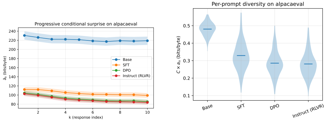
(a) AlpacaEval \bar{a}_k curves (length-matched).
