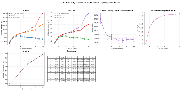
Figure 13. Summary metrics vs. mode count m (Qwen2.5-3B, n = 20 , 1000 draws). E_{\text{fit}} (sigmoid-extrapolated) increases monotonically, while the raw \hat{E}_n does not.
