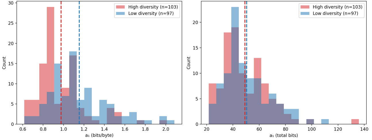
Figure 13. Distribution of a_1 (unconditional surprise of the first response) for high- vs. low-diversity story_gen samples. Left: per-byte. Right: total bits. The per-byte gap (see Table 7) is a dataset construction artifact.
