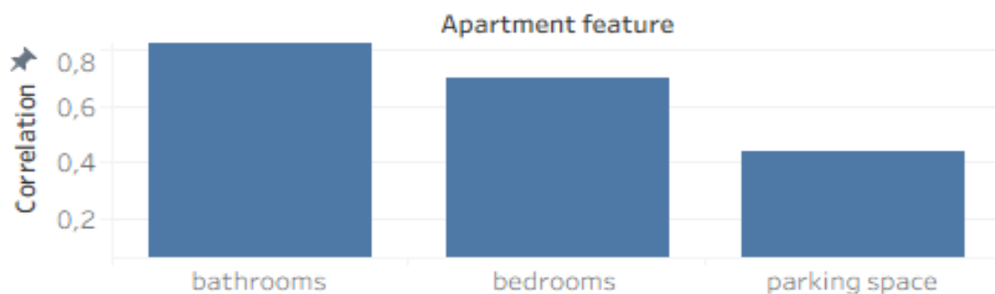
Relationship correlation of between each feature and monthly rental apartment price
