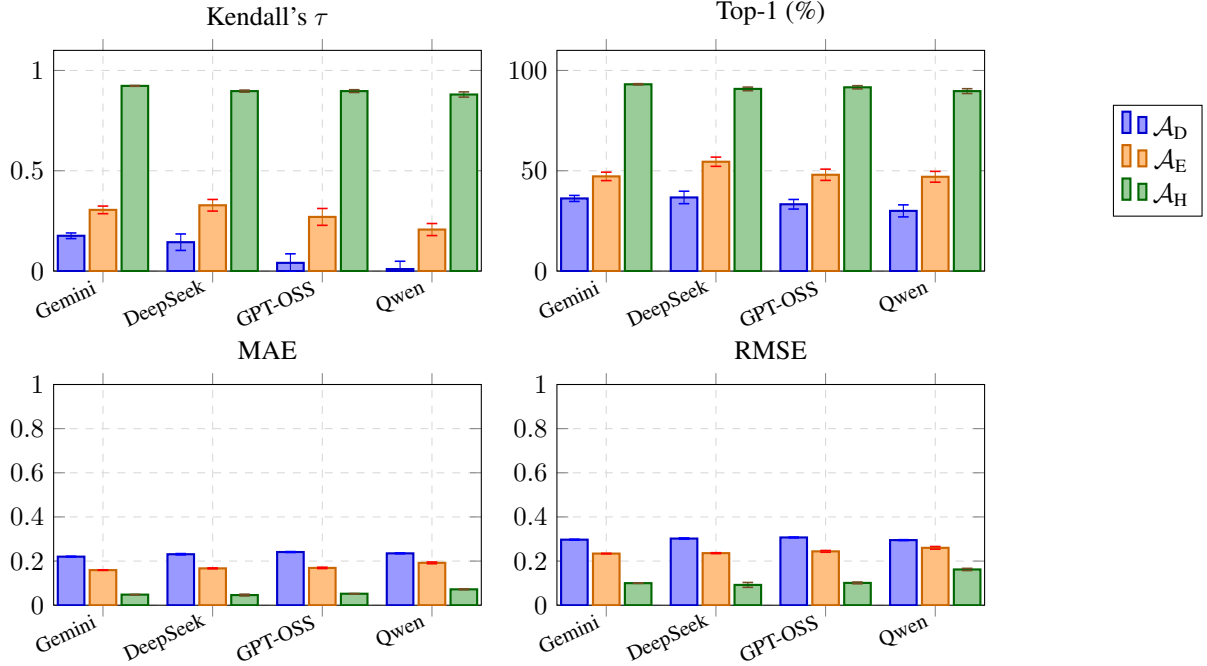
Figure 5: Overall performance by model (5-run mean \pm std, 195 scenarios). Error bars show \pm 1 std across five runs.
