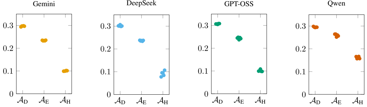
Figure H.13: Strip plots of Overall RMSE across five runs.
