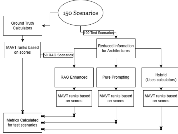
Figure 3: Decision-support workflow: scenario input \rightarrow architecture-specific scoring or extraction \rightarrow MAVT aggregation \rightarrow ranked output.
