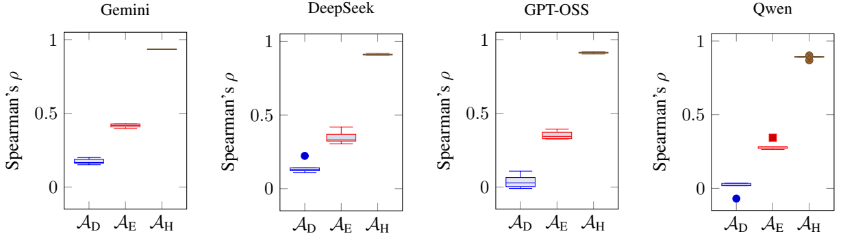
Figure 16: Distribution of Spearman's \rho across five independent runs per model.
