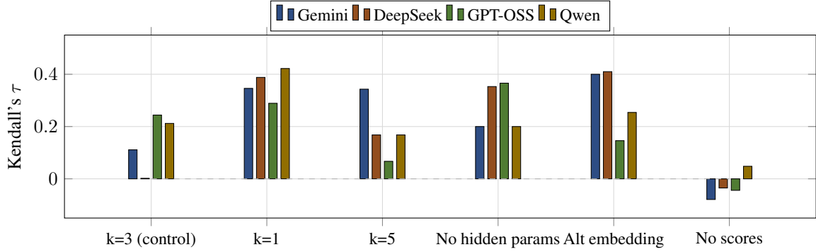
Figure 11: RAG ablation results: Kendall's \tau by configuration and model on the 12-scenario subset.
