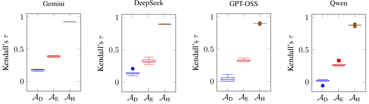
Figure 13: Distribution of Kendall's \tau across five independent runs per model. Box plots show median, quartiles, and whiskers.
