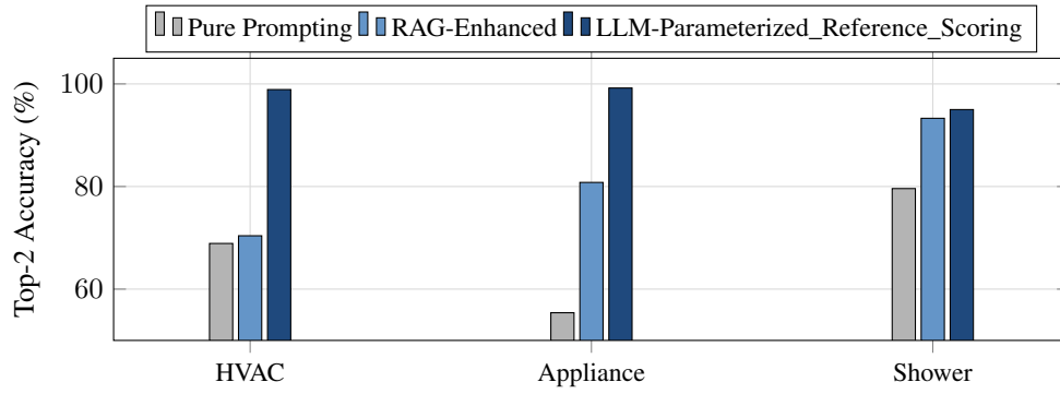
Figure 10: Top-2 accuracy by decision type and architecture. \mathcal{A}_H exceeds 95% on all types; \mathcal{A}_D remains below 80% on every type. Pooled across the four models; Section ?? confirms the architecture ordering holds individually per model.
