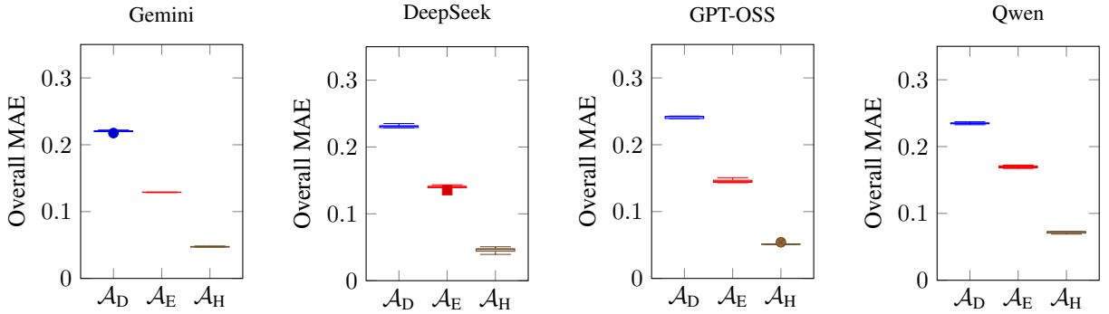
Figure 14: Distribution of Overall MAE across five independent runs per model.
