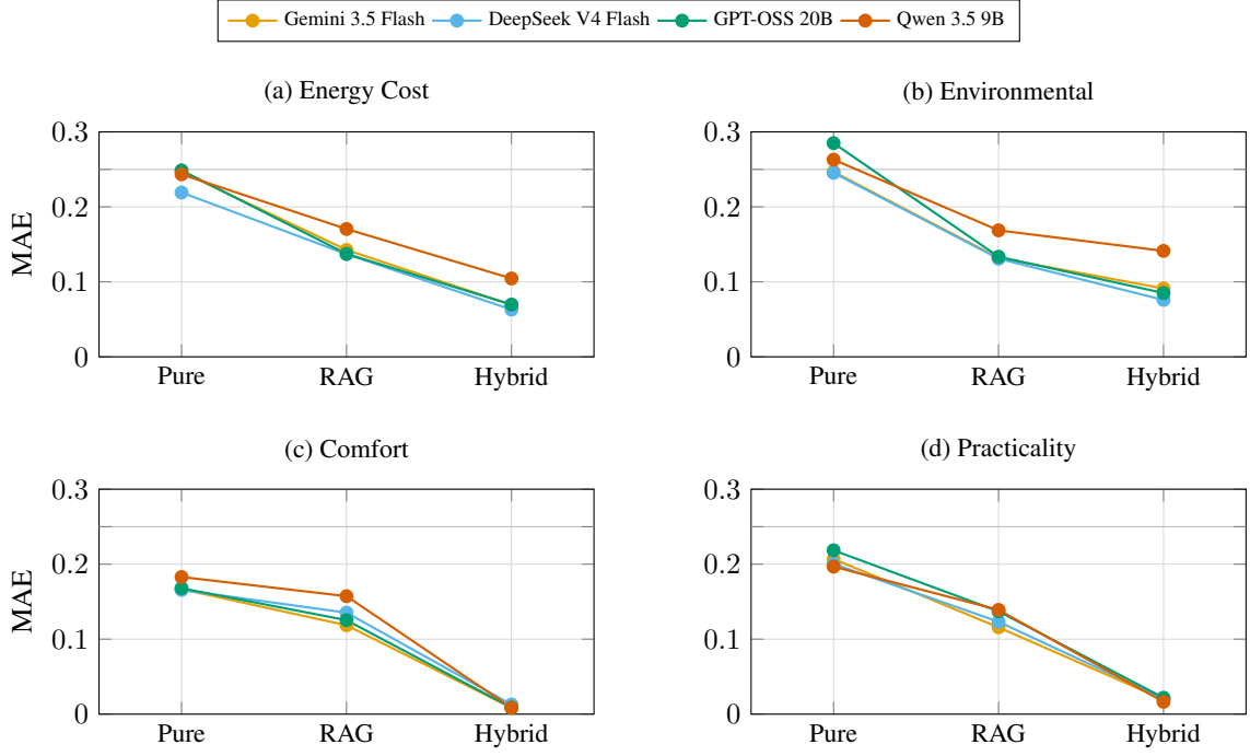
Figure 7: MAE by criterion and model (5-run mean, 195 scenarios each). Each line is one model; the x-axis is architecture (Pure \rightarrow RAG \rightarrow Hybrid).
