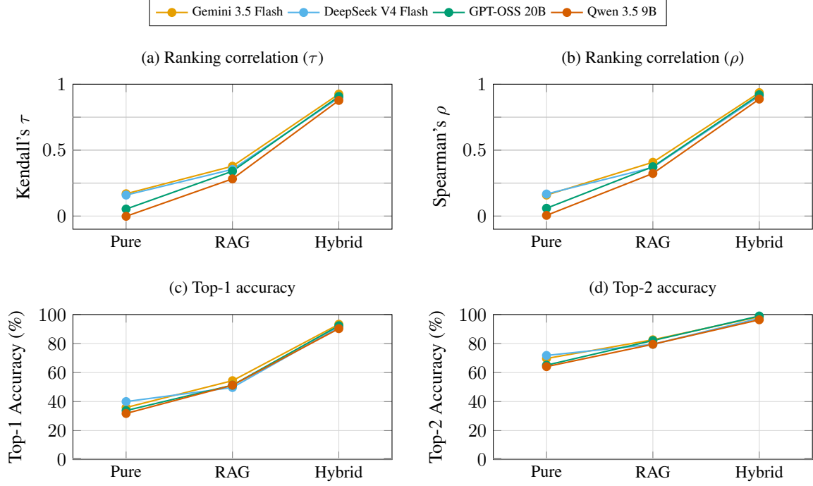
Figure 5: Ranking accuracy by model (5-run mean, 195 scenarios each). Each line is one model; the x-axis is architecture (Pure → RAG → Hybrid). Panels (a)-(b) and (c)-(d) intentionally use different y-axis scales, since rank correlation and percentage accuracy are not comparable units. Every model's line rises monotonically left to right, confirming the architecture ordering holds individually for all four models rather than only in a pooled average.
