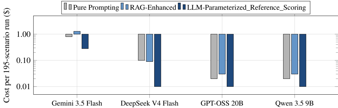
Figure 12: API cost per 195-scenario benchmark run by model and architecture. Note logarithmic y-axis; \mathcal{A}_H is the cheapest architecture across all four models.
