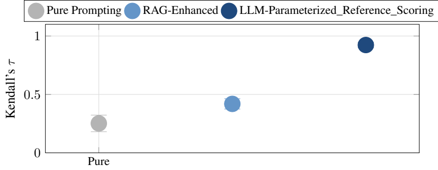
Figure 3: Kendall's \tau range for each architecture across the nine weight-perturbation scenarios (Table ??). The bands are non-overlapping, confirming that the architecture ordering ( \mathcal{A}_H > \text{RAG} > \text{Pure} ) is preserved under \pm 0.05 weight perturbations.
