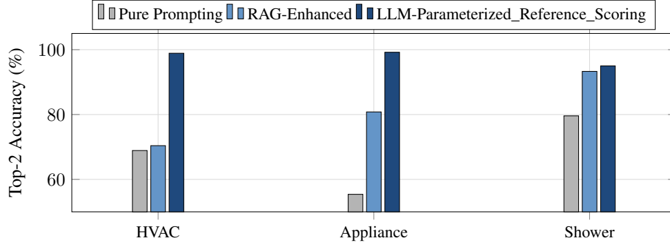
Figure 10: Top-2 accuracy by decision type and architecture. \mathcal{A}_H exceeds 95% on all types; \mathcal{A}_D remains below 80% on every type. Pooled across the four models; Section 5.1 confirms the architecture ordering holds individually per model.
