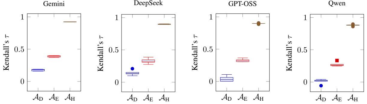
Figure 12: Distribution of Kendall’s \tau across five independent runs per model. Box plots show median, quartiles, and whiskers.
