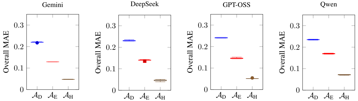
Figure 13: Distribution of Overall MAE across five independent runs per model.
