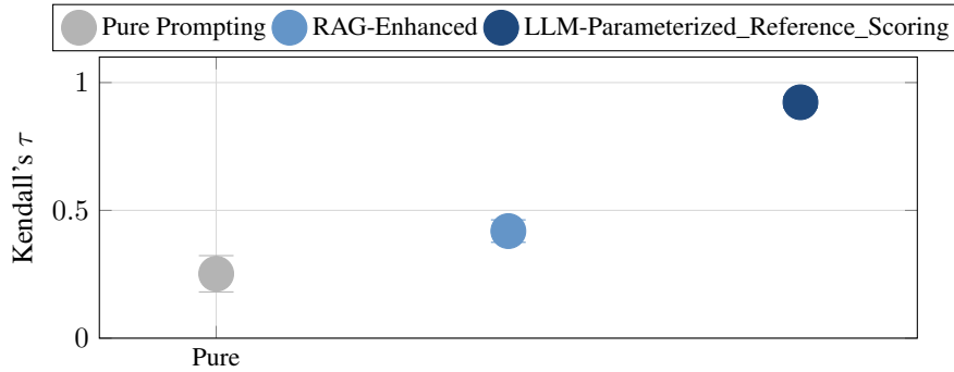
Figure 3: Kendall’s \tau range for each architecture across the nine weight-perturbation scenarios (Table 6). The bands are non-overlapping, confirming that the architecture ordering ( \mathcal{A}_H > \text{RAG} > \text{Pure} ) is preserved under \pm 0.05 weight perturbations.
