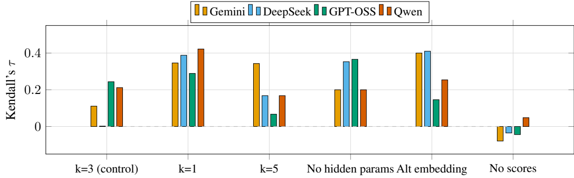
Figure 11: RAG ablation results: Kendall's \tau by configuration and model on the 12-scenario subset.
