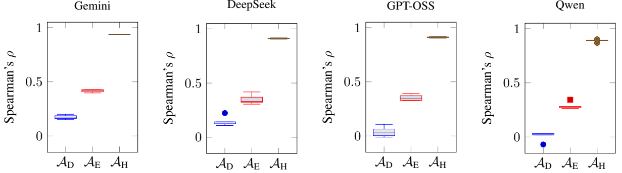
Figure 15: Distribution of Spearman's \rho across five independent runs per model.
