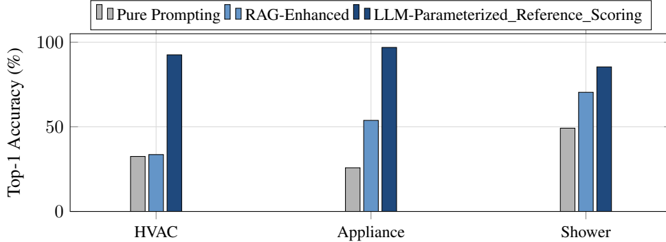
Figure 9: Top-1 accuracy by decision type and architecture. \mathcal{A}_H exceeds 85% across all three decision types; \mathcal{A}_D fails to surpass 50% on any type. Pooled across the four models; Section 5.1 confirms the architecture ordering holds individually per model.
