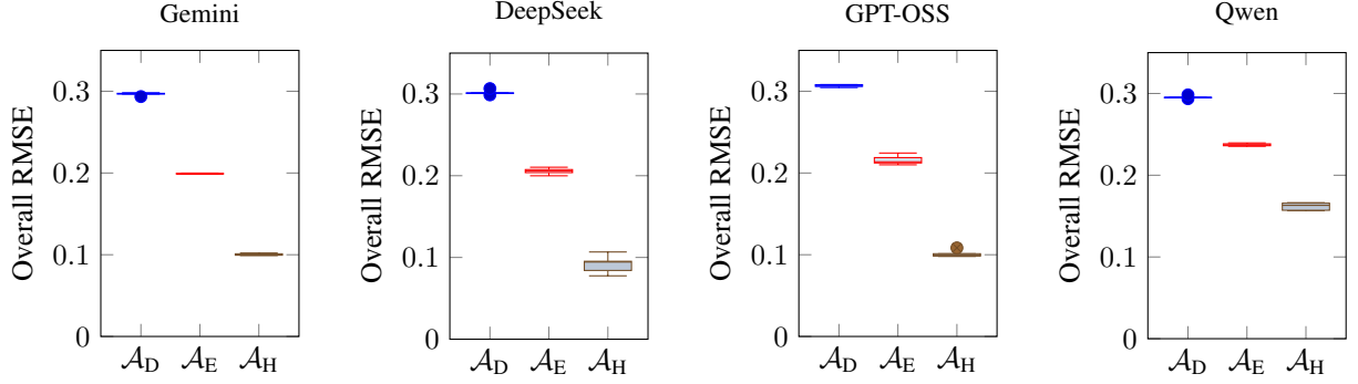
Figure 16: Distribution of Overall RMSE across five independent runs per model.
