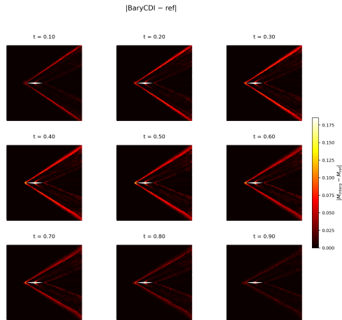
Barycentric CDI (det)
