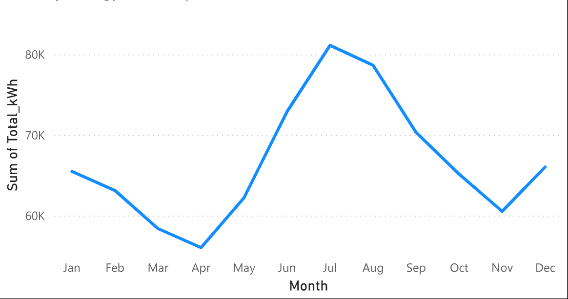
Monthly Energy Consumption (kWh)
