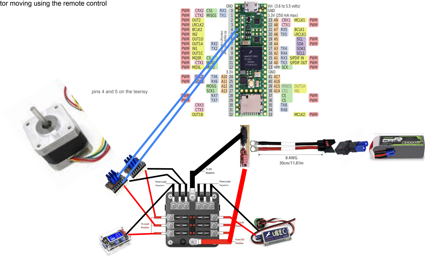
The staging motor moving using the remote control
