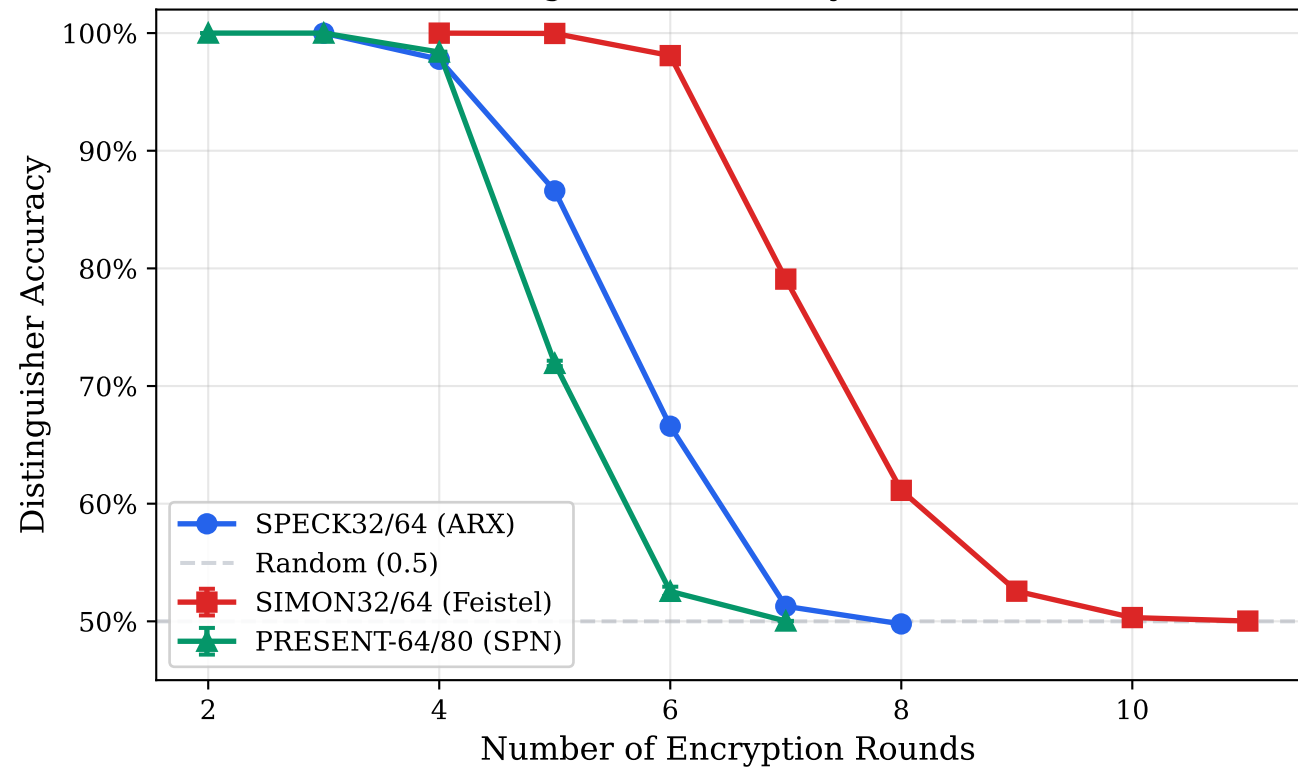
Neural Distinguisher Accuracy vs. Round Count
