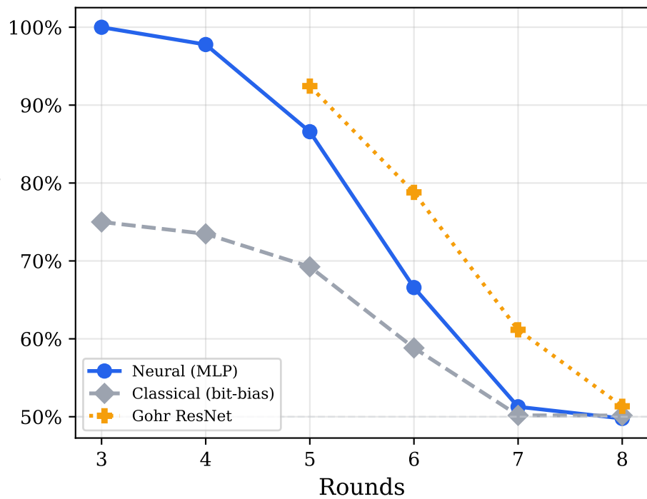
SPECK32/64 (ARX)
