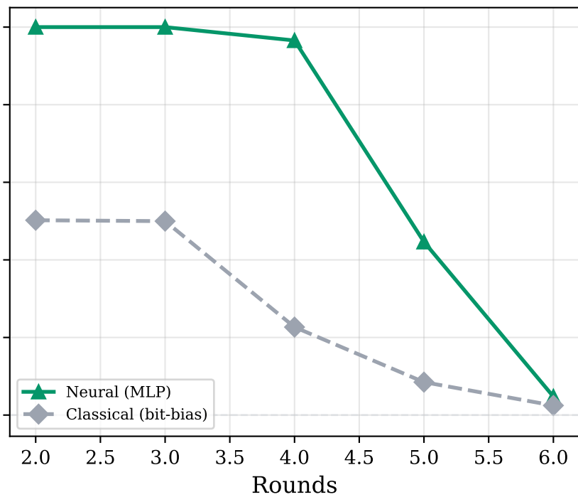
PRESENT-64/80 (SPN)
