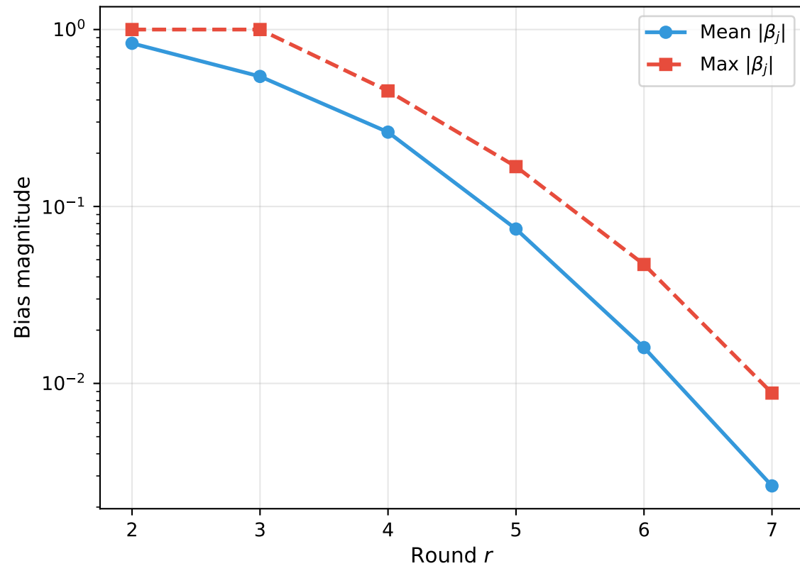
PRESENT (SPN)
