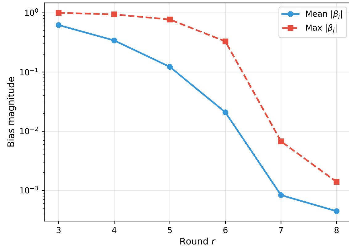
SPECK32/64 (ARX)
