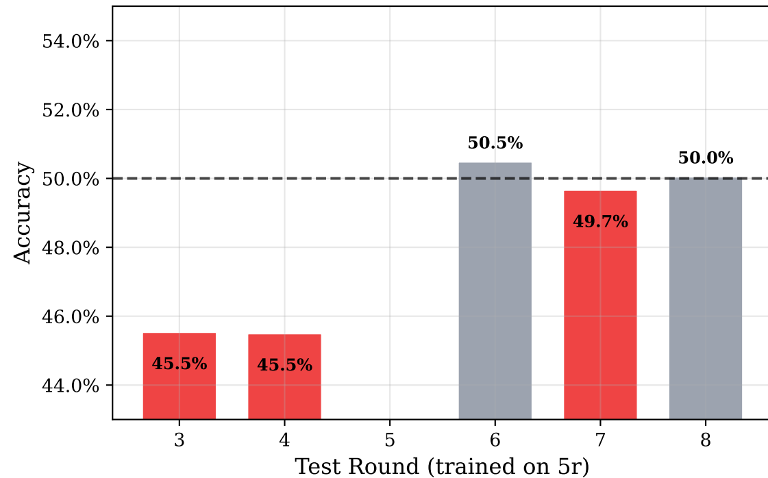
SPECK32: Cross-Round Transfer
